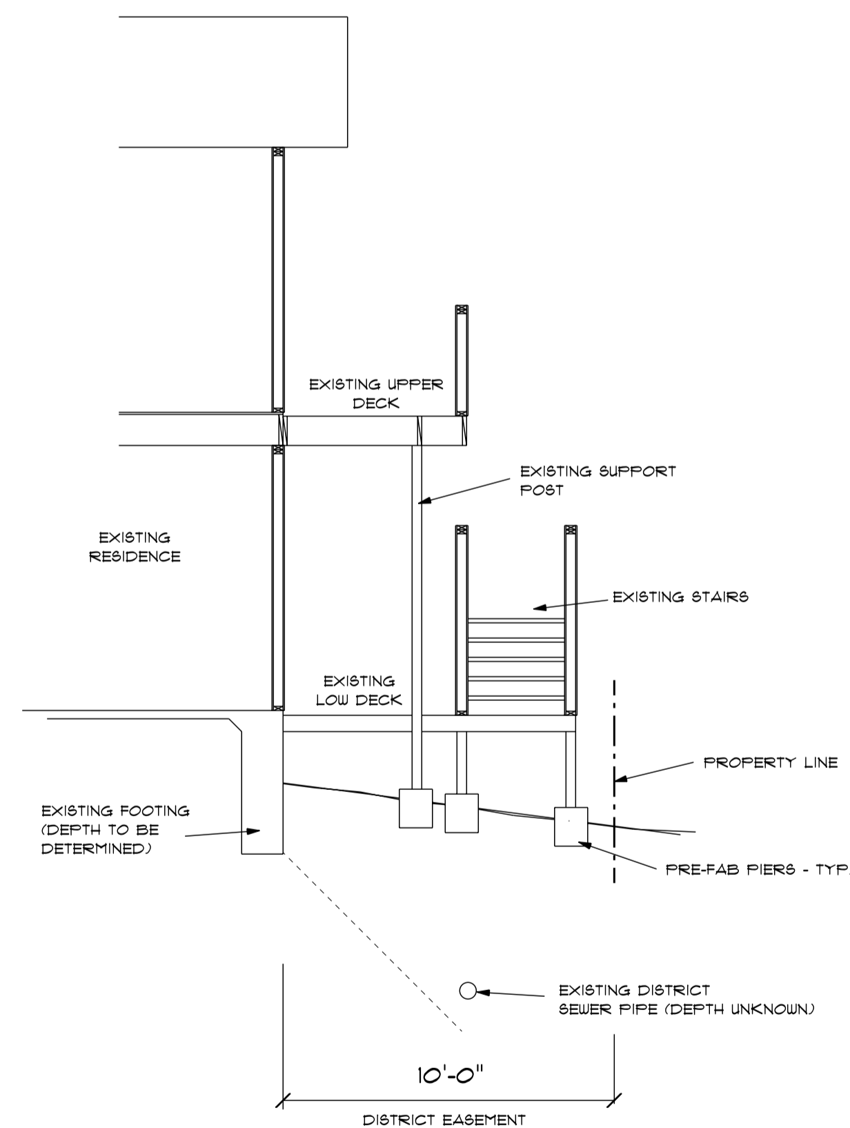
AS-BUILT SECTION A
